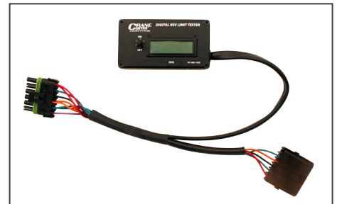
Digital Rev Limit Ignition Tester Part #1000-1050
